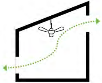
FIGURE 9 Diagram of convection ventilation in section with high-level and low-level operable windows
