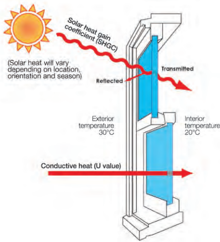
FIGURE 13 Key Properties of Glass SOURCE: Your Home 7
