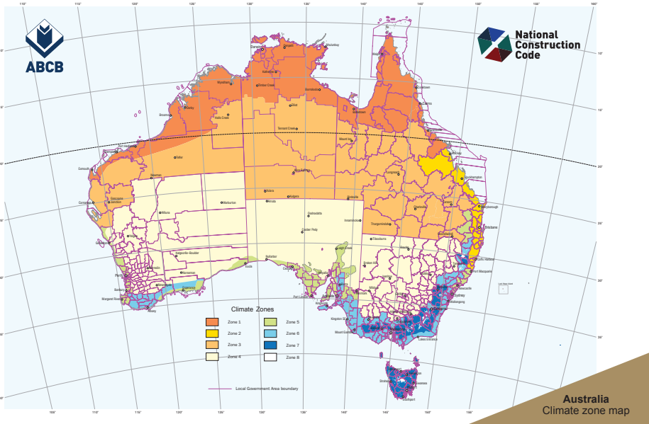
FIGURE 29 Climate Zone Map Australia SOURCE: Australian Building Codes Board (ABCB)
